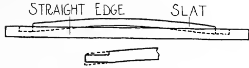
FIG. 404. LAYING OFF TENONS ON CURVED STOCK.
